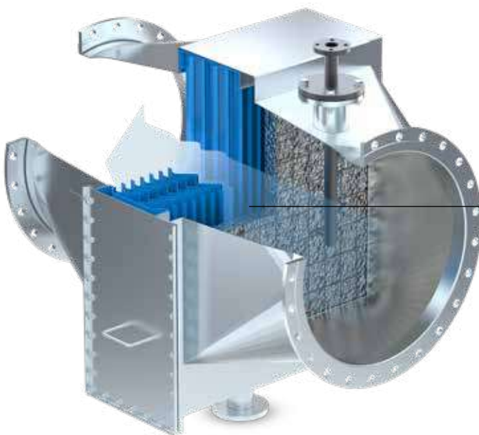
Housing with mist eliminator for horizontal gas flow (Type LTH 600) and agglomerator
