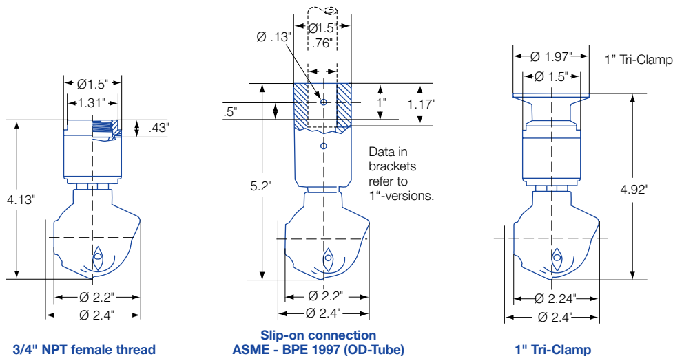
3/4" NPT female thread
