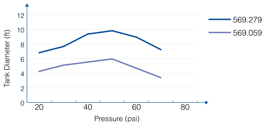
Overview of the tank diameter, depending upon the pressure of series 569
